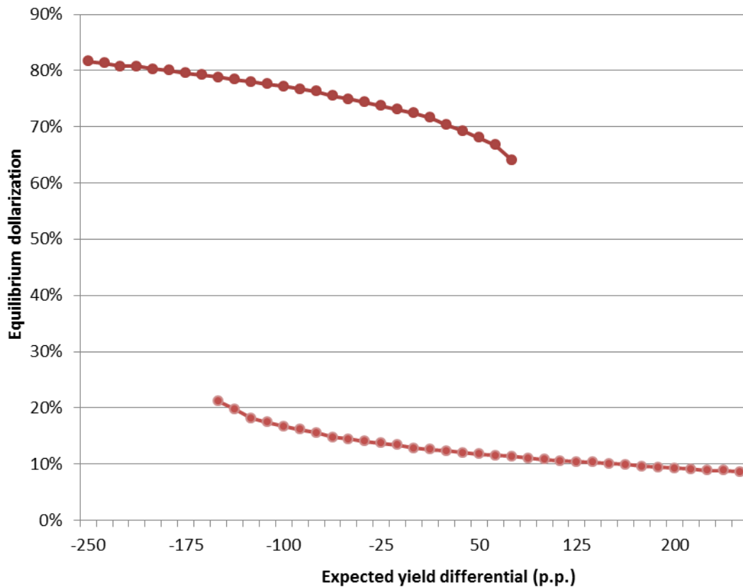
Figure 2. Dollarization equilibria
