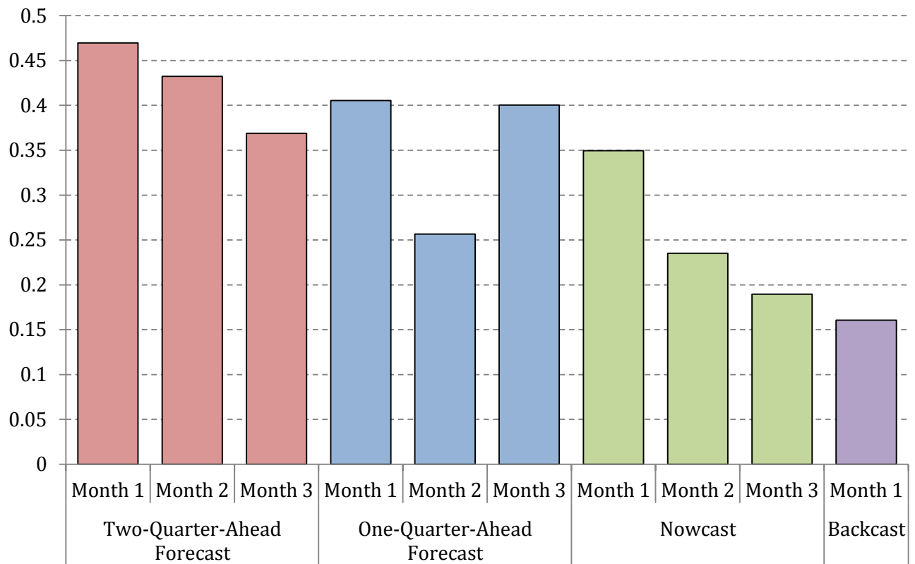
Figure 2. Average RMSEs
