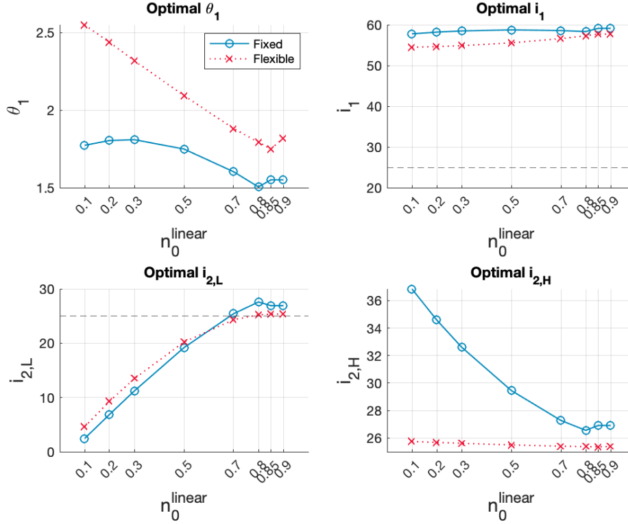
Figure 5: Supplemental Result 2 – change in n_0^{linear}
